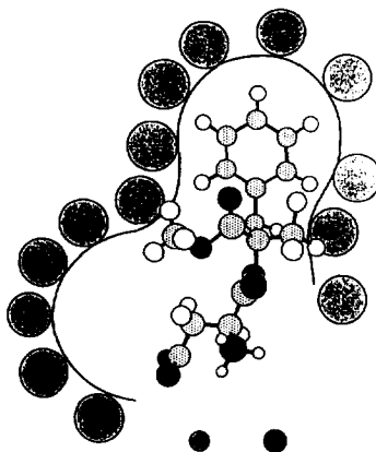
Figure 1. Fit of the X-ray diffraction molecular structure of the aspartame analogue 7 11 in the model of the active site of the sweet receptor. 12,16,17 The conformation is F I D II , identical to the proposed bioactive conformation of aspartame. As for aspartame, the ester group sticks out of the main plane of the active site. The donor and acceptor moieties of the AH-B entity of the receptor are represented as a nitrogen and an oxygen atom, respectively.
