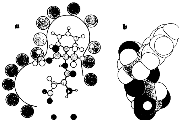
Figure 2. (a) Fit of the minimum energy conformer of the aspartame analogue 3 in the model of the active site of the sweet receptor. 12,16,17 Both the ester and the C α -methyl groups stick out of the main plane of the active site. The donor and acceptor moieties of the AH-B entity of the receptor are represented as a nitrogen and an oxygen atom, respectively. (b) The same conformer of 3 represented as a space-filling model in a direction parallel to the plane of the bidimensional contour.
