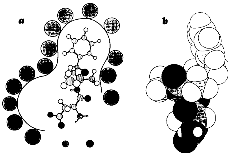
Figure 3. (a) Fit of the minimum energy conformer of the aspartame analogue 11 in the model of the active site of the sweet receptor. 12,16,17 Both the ester and the C α -methyl groups stick out of the main plane of the active site. The donor and acceptor moieties of the AH-B entity of the receptor are represented as a nitrogen and an oxygen atom, respectively. (b) The same conformer of 11 represented as a space-filling model in a direction parallel to the plane of the bidimensional contour.
